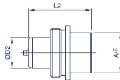
PSP SERIES POPPET COUPLING
