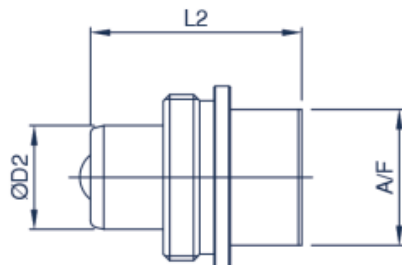
PSB SERIES BALL COUPLING
